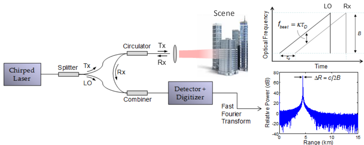
Figure 1. A conceptual diagram of FMCW lidar.
