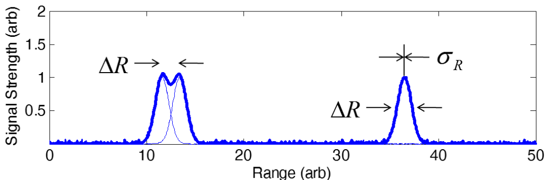
Figure 2. A conceptual diagram of FMCW lidar.
